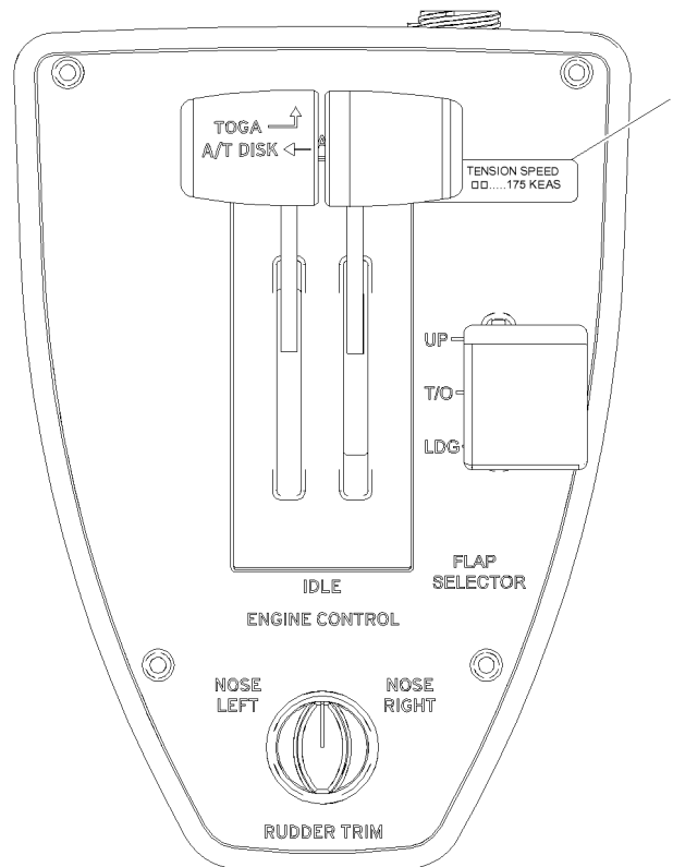
Speed Restriction Placard Location on Throttle Quadrant Figure 1 (Sheet 1 of 1)
